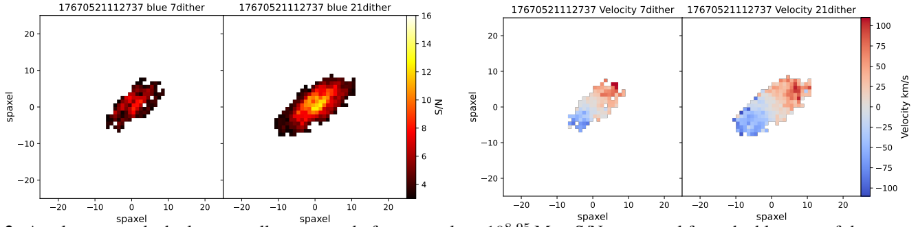
Figure 2: A galaxy towards the lowest stellar mass end of our sample at 10^{8.95} M_{\odot} . S/N per spaxel from the blue arm of the spectrograph for spaxels with S/N > 3 (left pair) and H-alpha velocity (right pair) for the improved 21-dither strategy (right of each pair) compared to the 7-dither strategy (left of each pair). Stellar kinematics would have been impossible on a significant sample of such low-mass galaxy before Hector. Hector is achieving the required S/N > 3 in 80% more spaxels using the 21-dither observations rather than the standard 7-dithers. This means complex kinematics can be mapped across the galaxy not possible in the patchy few central spaxels detected in 7 dithers.
