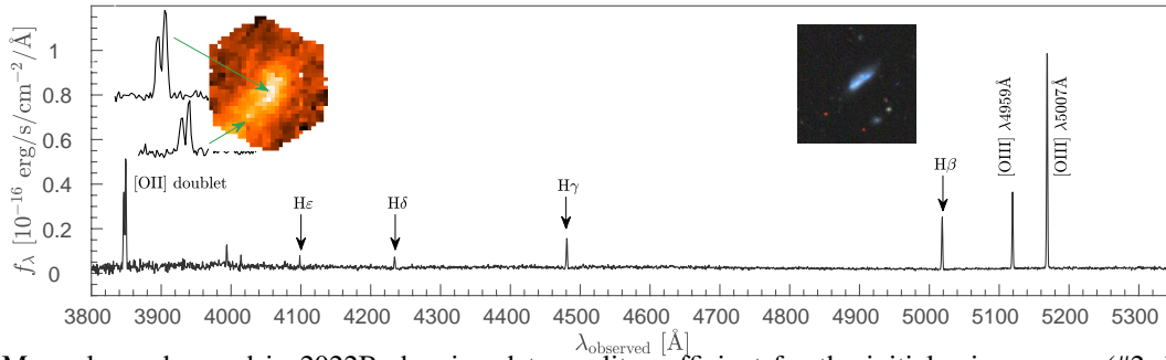
Figure 1: A 10^{8.8}M_{\odot} galaxy observed in 2022B showing data quality sufficient for the initial science case (#2, below) ‘Inflows and outflows at large radii’. This is at the most challenging, lowest mass end of the Hector selection, yet strong emission lines are detected with de-blending of the [OII] doublet lines in spaxels right out to the edges of the hexabundle. The spectrum is from Hector’s Spectrograph blue arm; the left inset is the Hector reconstructed image highlighting the continuum and [OII] doublet in two spaxels; the right inset is the optical Dark Energy Camera Legacy Survey (DeCALs) image.
