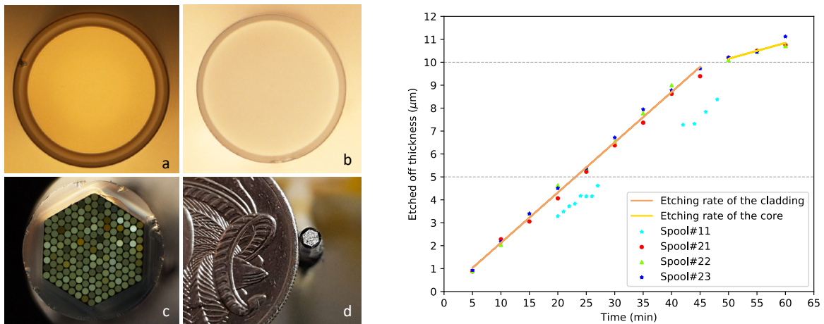
Figure 1: Single optical fibres (top left) used to make the 169-core hexabundle (bottom left) as discussed in the text. Right: Fibres from Spool#11 are made with PCVD+POVD which have a slower etching speed.
